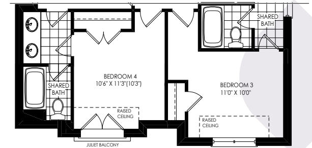
OPT. 5 BEDROOM SECOND FLOOR ELEVATION B
